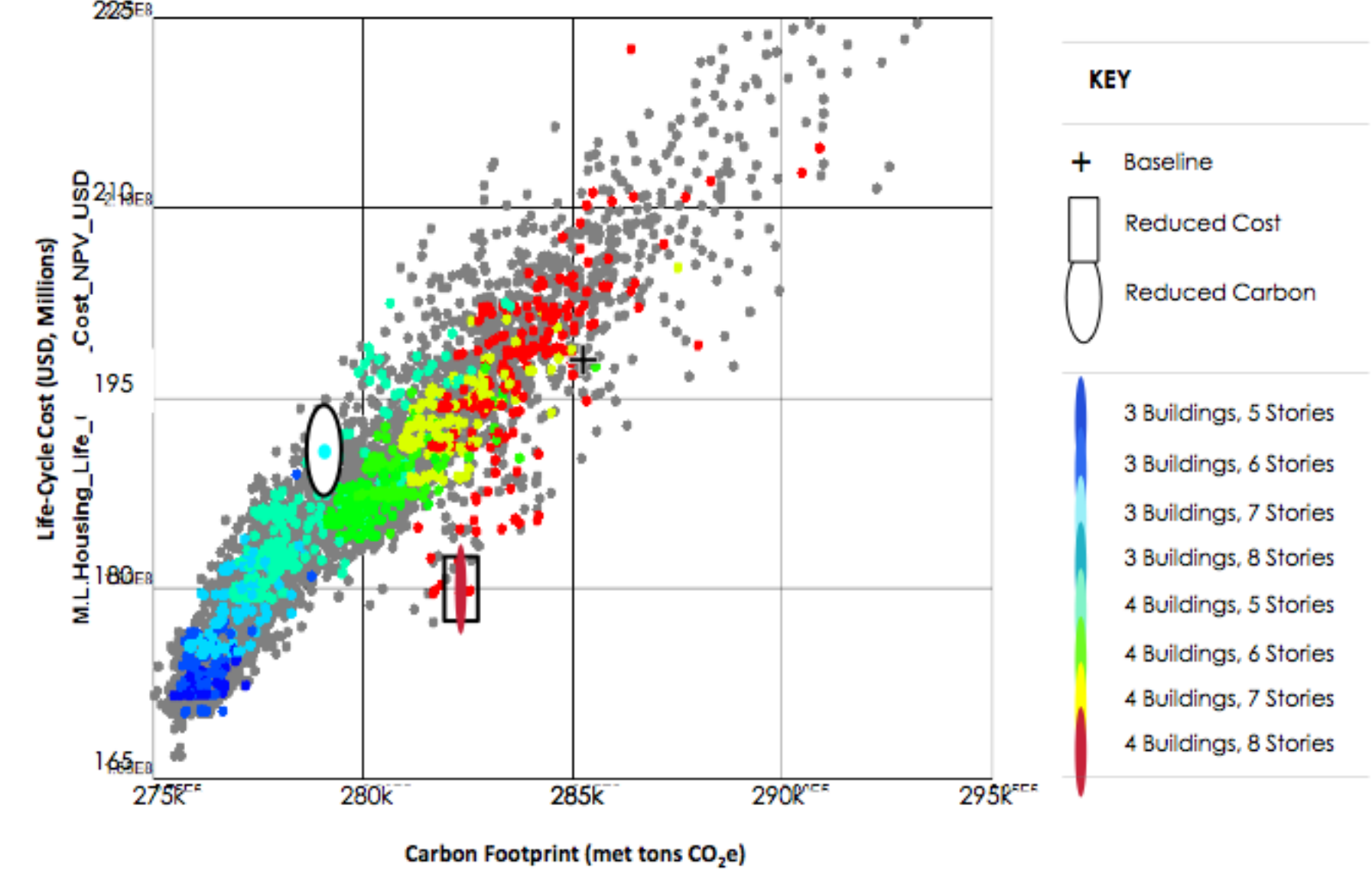
Results: Life-Cycle Cost vs. Carbon Footprint
