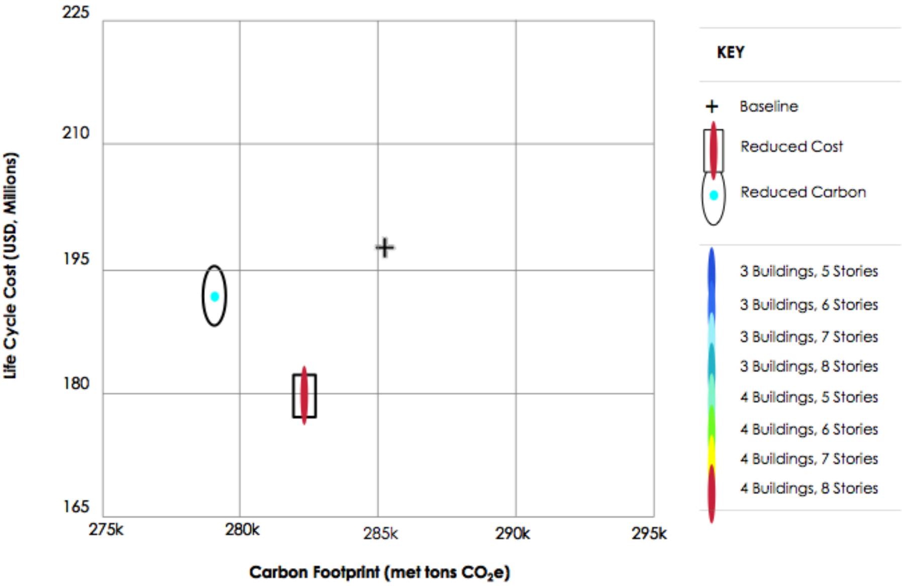
Life-Cycle Cost vs. Carbon Footprint: 3 Designs
